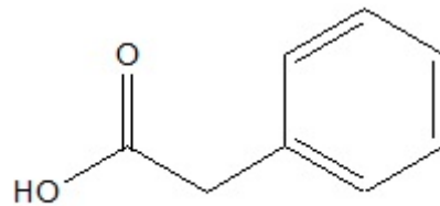
Phenylacetic acid
