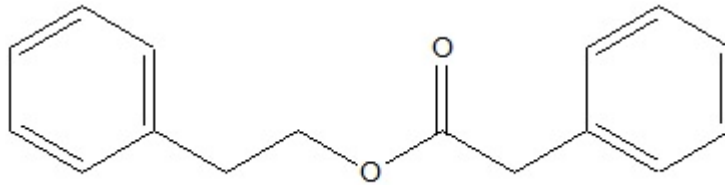
Phenylethyl phenylacetate
